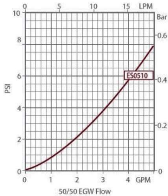
Liquid Side Pressure Drop - EGW
