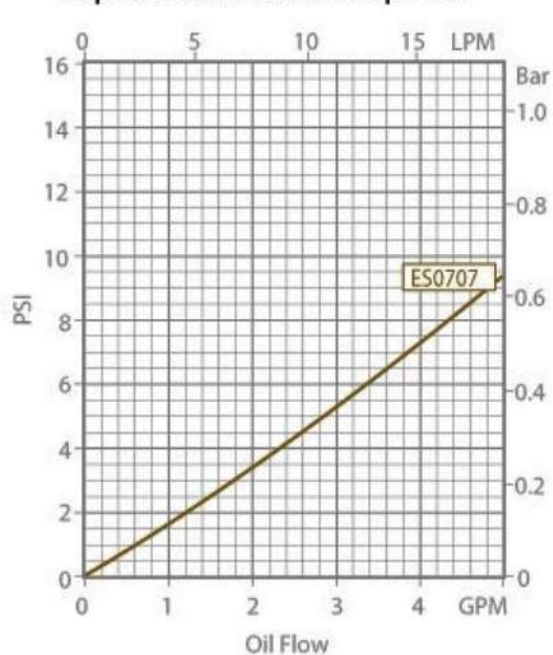
Liquid Side Pressure Drop - Oil
