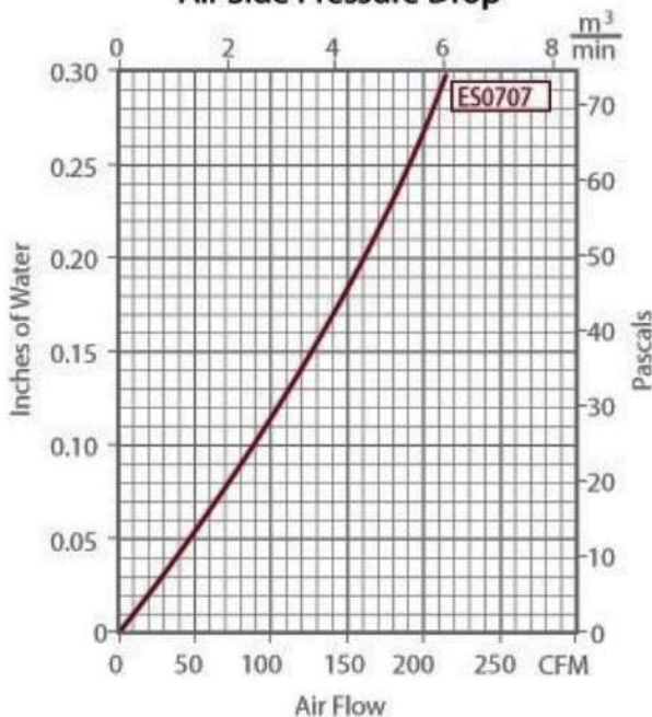
Air Side Pressure Drop
