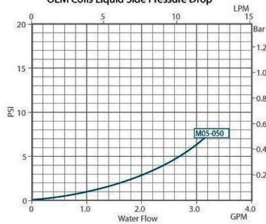
OEM Coils Liquid Side Pressure Drop
