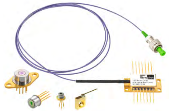
nanoplus DFB lasers on TO66, TO5, TO5.6, c-mount and SM-BTF
