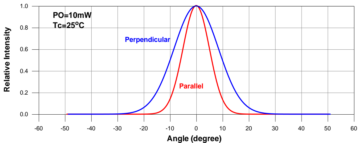
Far-Field Pattern
